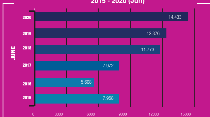
Historical motorcycle sales (units) 2015 - 2020 (Jun)
