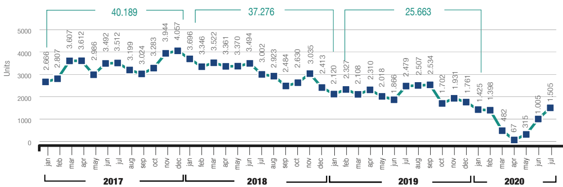
Monthly sales of assembled vehicles in Ecuador (units)
