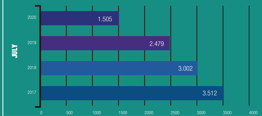
Historical sales of assembled vehicles (units) 2017 - 2020 (July)
