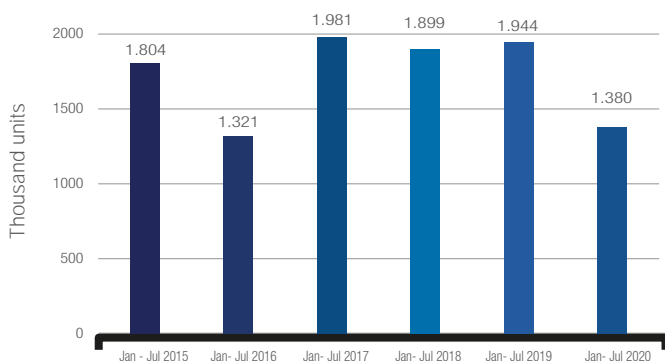
Total tires imports* (thousand units) 2015 - 2020 (Jan - Jul)
