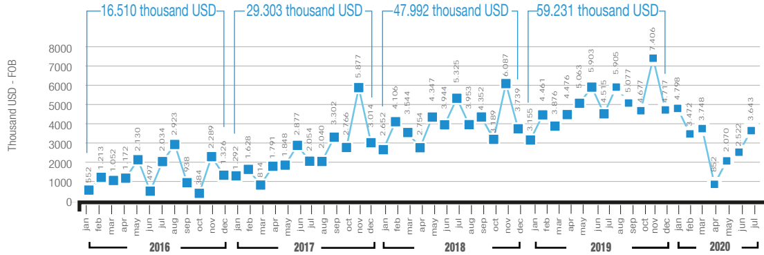
Monthly motorcycle imports (thousand USD - FOB)
